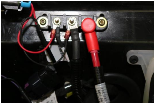
Newer RZR Busbar's have Battery and Ground attached.
